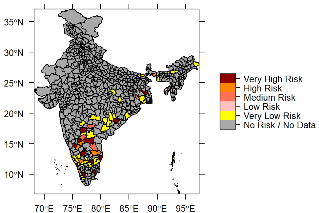
Risk Prediction of Anthrax for the month of March 2019
